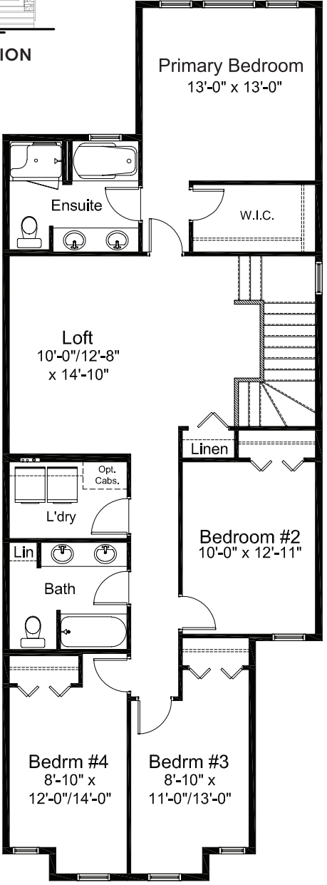
UPPER FLOOR 1,380 sq. ft.
