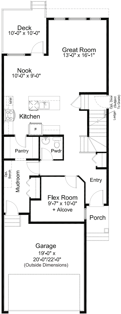
MAIN FLOOR 992 sq. ft.
