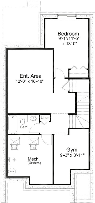
Basement Development Option 683 sq. ft. of developed area
