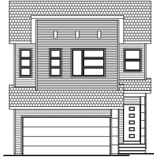
INTERNAL STREET ELEVATION
