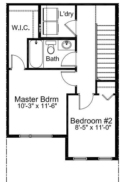
UPPER FLOOR: 515 SQ. FT.
